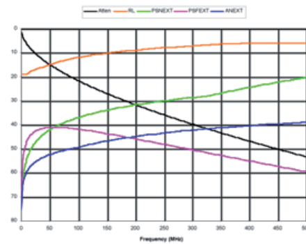
Figure 2(a): Category 6 cabling to 500 MHz
